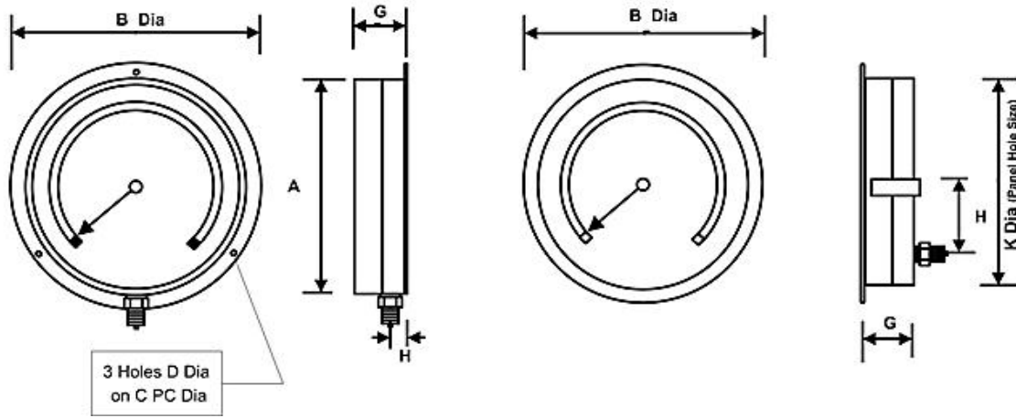
Flush Clamp Mounting
